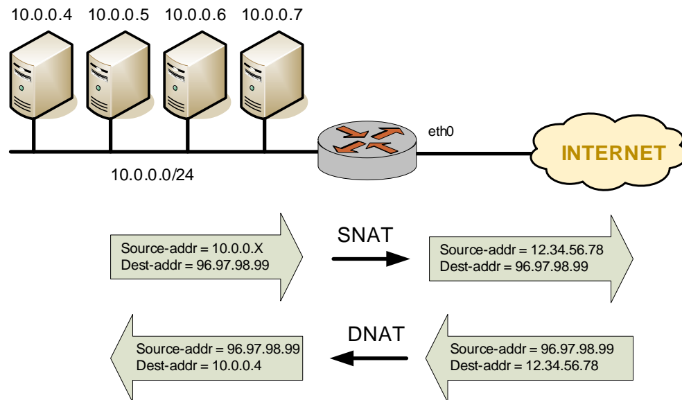
Figure 2-9 Bidirectional NAT
