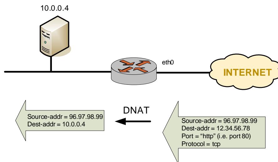
Figure 2-6 Destination NAT (one-to-one)
