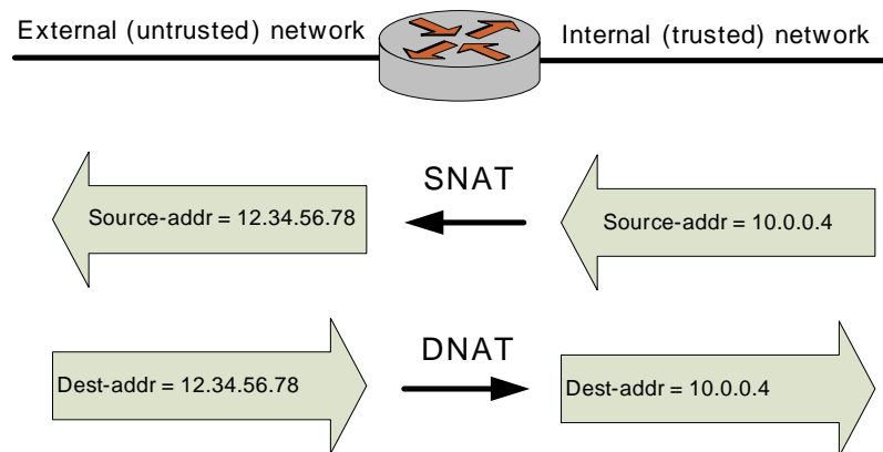
Figure 1-6 Bidirectional NAT
